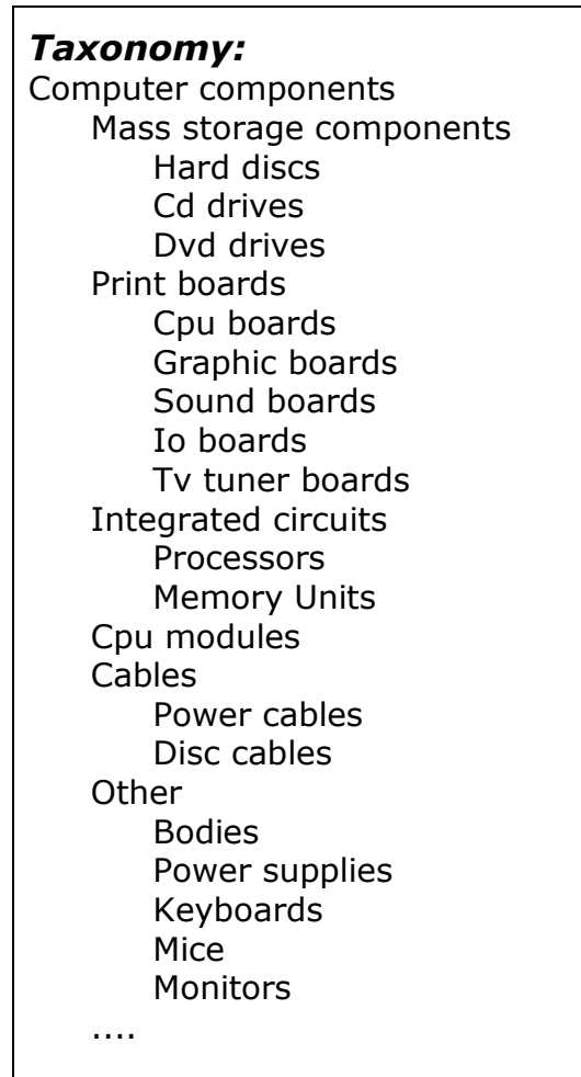
Figure 5 - Sample taxonomy of computer components
